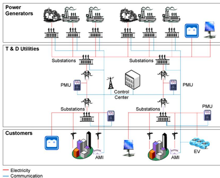
Figure 2 Smart Grid
