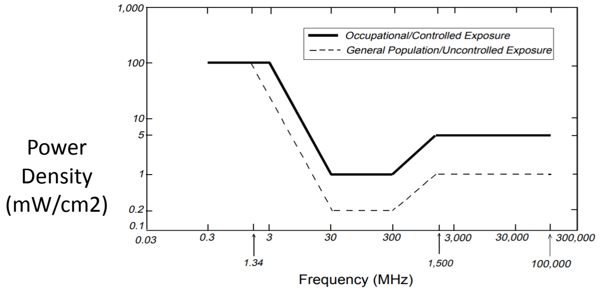
Figure 1. FCC Limits for Maximum Permissible Exposure (MPE) Plane-wave Equivalent Power Density
